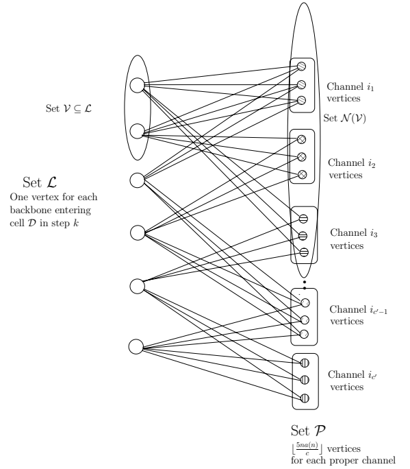
Figure 4: Bipartite Graph for Cell D in step k
