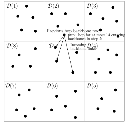
Figure 3: Cell D and neighboring cells during backbone construction
