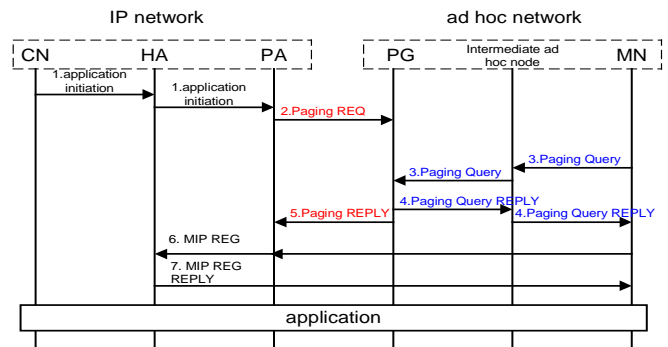
Figure 1: Message flows of Reactive Paging
