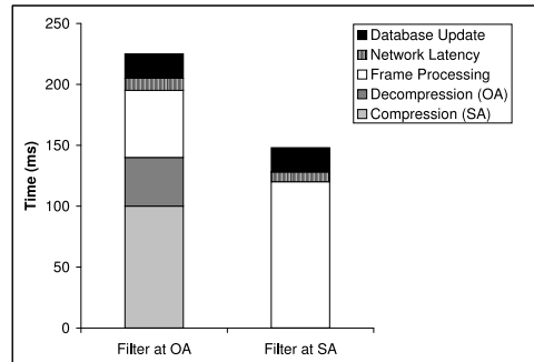
Figure 1: Sensor feed processing time
