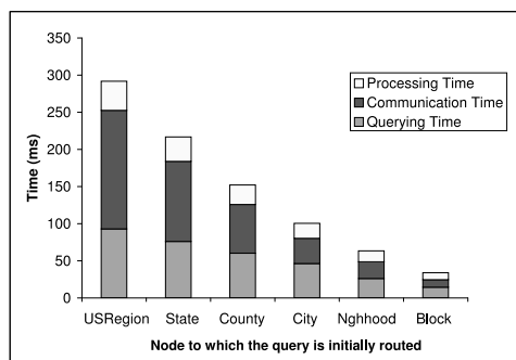
Figure 3: Query processing time
