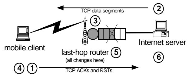
Figure 2. The Fast Reset algorithm.
