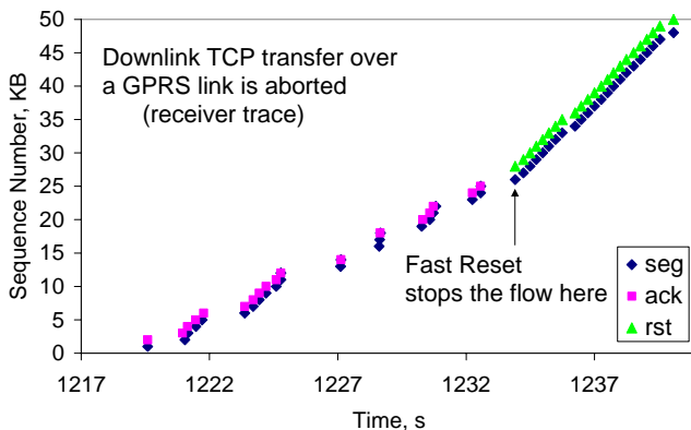
Figure 1. Aborted TCP connection over GPRS to www.zed.com (Mozilla/HTTP 1.1).
