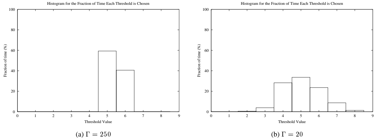
Figure 7: Figures (a) and (b) plot the fraction of time each threshold is chosen by \Delta_O(\Gamma) in topology 1 for \Gamma equal to 250 and 20, respectively. Here, \lambda_M = 50 packets/sec and \lambda_U = 500 packets/sec.
