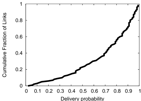
Figure 4: The distribution of delivery probabilities of links used in Srcr routes, at the bit-rates chosen by SampleRate. The median is 0.8, meaning that Srcr often uses links with loss rates of 20% or more. (multi-hop TCP, loss matrix)
