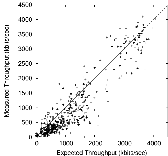
Figure 10: Comparison of multi-hop throughput and throughput predicted from individual hop throughputs. Each point represents one node pair. The expected throughputs for single-hop routes (most of the points above 2000 kbits/second) differ from the measurements, but the errors are not biased, since the predictions are themselves a separate set of measurements. The expected multi-hop throughputs are mostly higher than the measured throughputs. (multi-hop TCP and simulations from single-hop TCP)
