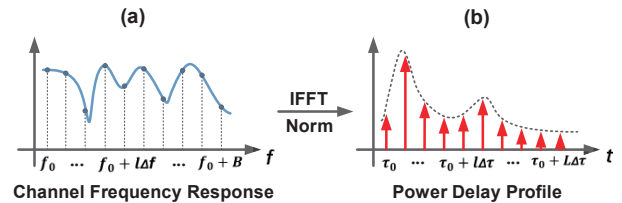
Figure 1: Transformation from a channel frequency response to the power delay profile. (a) A channel frequency response, where f_0 , \Delta f , and B represent starting frequency, frequency sampling resolution, and bandwidth, respectively; (b) Derived power delay profile, where \tau_0 and \Delta\tau represent the propagation delay of LoS path and the power delay profile resolution, respectively.
