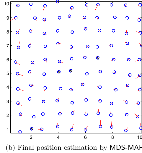
Figure 9: Estimation on the grid network using neighbor distances with 5% error.
