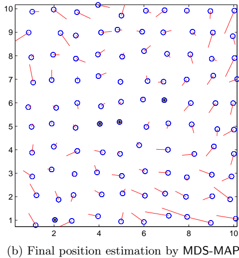
Figure 8: Estimation on the grid network using connectivity information only.
